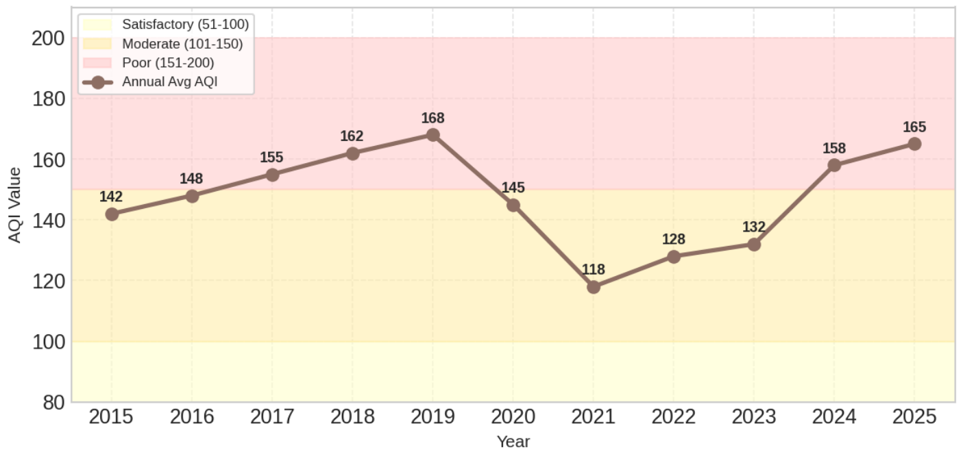
Prayagraj Estimated AQI Decadal Trend (2015–2025)
